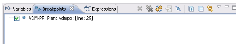
Figure 3.13: Breakpoint View
